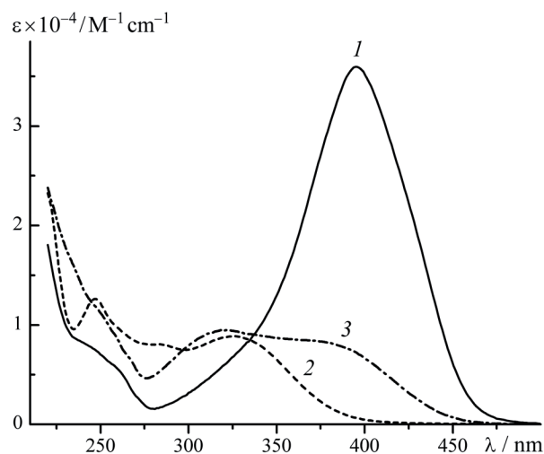
Figure 5. Absorption spectra of complexes ( trans - 34a ) \cdot\text{Mg}^{2+} (1), ( cis - 34a ) \cdot\text{Mg}^{2+} (2) and ( cis - 34a ) \cdot(\text{Mg}^{2+})_2 (3) in MeCN, as measured at a concentration of 2 \times 10^{-5} M.
