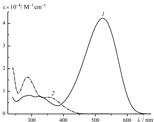
Figure 6. Absorption spectra of two isomeric forms of dye 39 in MeCN: 1 – trans -isomer, 2 – cis -isomer.
