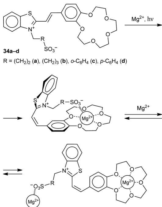
Scheme 2. Synthesis of complexes ( cis - 34a ) \cdot\text{Mg}^{2+} and ( cis - 34a ) \cdot(\text{Mg}^{2+})_2 .
