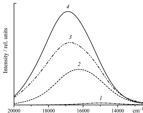
Figure 4. Corrected luminescence spectra of dye 26 (1) and complexes \text{26}\cdot\text{Ca}^{2+} (2), \text{26}\cdot\text{Sr}^{2+} (3) и \text{26}\cdot\text{Ba}^{2+} (4) in MeCN; the spectra are normalized so that the integral intensities are directly proportional to the luminescence quantum yields; the quantum yields are 0.0013 ( 26 ), 0.029 ( \text{26}\cdot\text{Ca}^{2+} ), 0.056 ( \text{26}\cdot\text{Sr}^{2+} ) and 0.078 ( \text{26}\cdot\text{Ba}^{2+} ).
